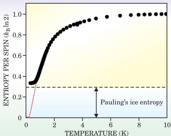
Figure 3. The entropy S of the spin-ice compound dysprosium titanate \text{Dy}_2\text{Ti}_2\text{O}_7 , as a function of temperature T . At high T , S = k_B \ln 2 per spin, the same as for free spins. Cooling the system causes the entropy to drop as correlations develop between spins. An unfrustrated magnet follows the plot's schematic red line down to zero entropy because the system assumes a unique ground state. In spin ice, geometrical frustration creates an exponentially large number of degenerate ground states. The large degeneracy manifests itself in a nonvanishing entropy, which is close to the value that Linus Pauling predicted for ordinary water ice. (Adapted from ref. 5.)
