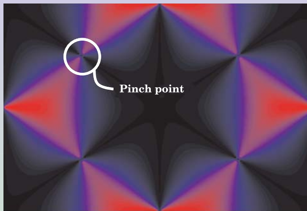
Figure 5. Fourier transform of the spin correlations in a high-symmetry plane of the frustrated pyrochlore magnet. Red regions denote strong correlations; black regions, weak ones. The local constraint on the sum over spins in a tetrahedron leads to the appearance of bow-tie motifs. These each have a pinch point at their center, which is a location of discontinuity but not divergence; the value of the spin correlations in the vicinity of those pinch points depends on the direction, but not on the distance, that one moves away from them. Back in real space, the ground-state constraint on the spins leads to algebraic correlations of the dipolar type, (3\cos^2\theta - 1)/r^3 . (Courtesy of Sergei Isakov.)
