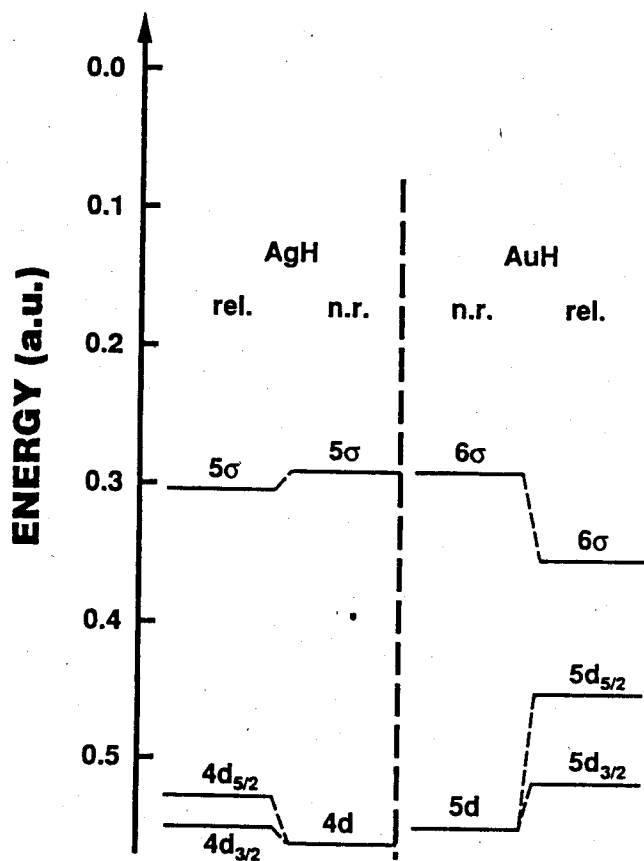
Figure 1. Orbital energies of the diatomic molecules \text{AgH(g)} and \text{AuH(g)} from relativistic and nonrelativistic calculations. Energies in atomic units, 1 a.u. = 27.212 eV = 2625.5 kJ mol -1 . Thus \Delta E \approx 260 kJ per step of the ordinate axis. Adapted from Pyykkö (9).
