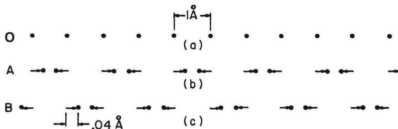
Figure 1: (a) The rigid lattice of polyacetylene; (O) the carbon atoms are equally spaced 1\text{\AA} apart. (b), (c) The effect of Peierls’ instability is to shift the carbon atoms .04\text{\AA} to the right (A) or to the left (B), thus giving rise to a double degeneracy.
