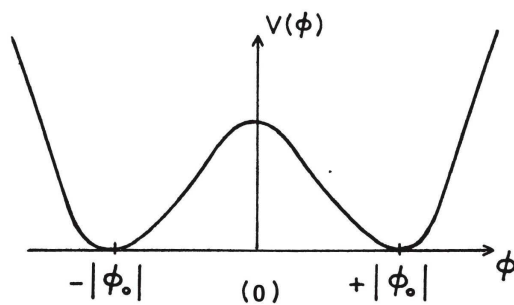
Figure 2: Energy density V(\phi) , as a function of a constant phonon field \phi . The symmetric stationary point, \phi = 0 , is unstable. Stable vacua are at \phi = +|\phi_0| , (A) and \phi = -|\phi_0| , B.
